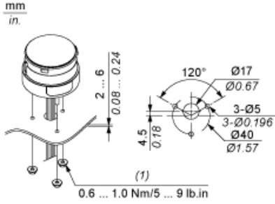
(1) M4 Nut x 3 (attached)
